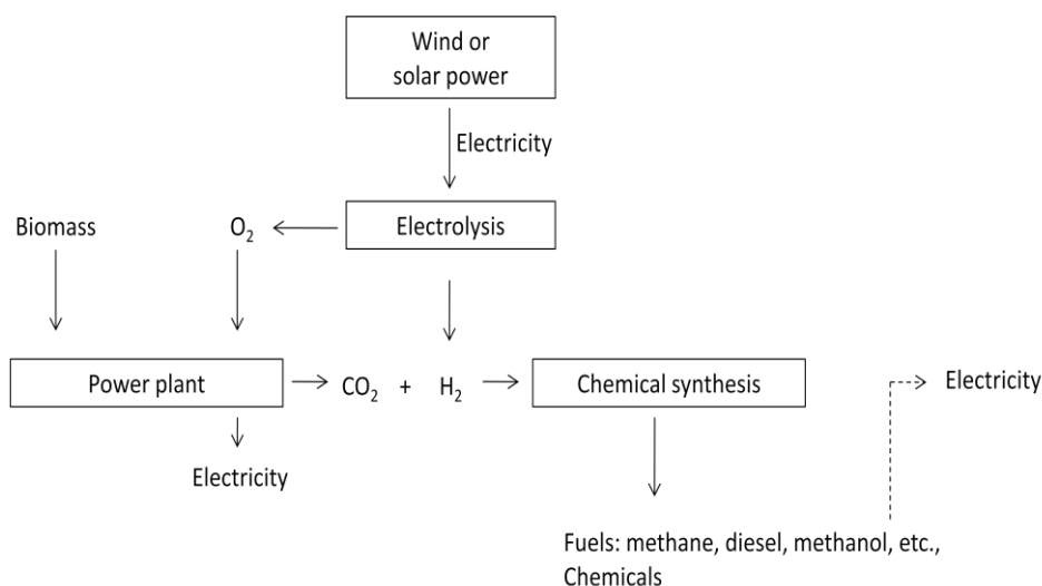
Figure 1. Carbon Capture and Recycling, CCR using the oxygen from electrolysis in an oxy-fuel combustion of the biomass, and capturing the biogenic CO 2 from the biomass combustion by the hydrogen from electrolysis
